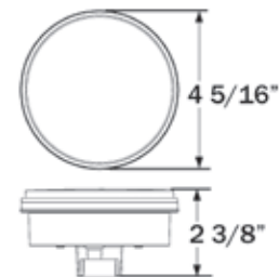
HOLE CUT-OUT: 4.5"
