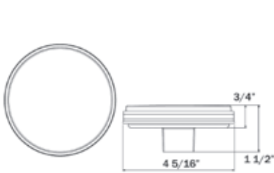
HOLE CUT-OUT: 4.5"
