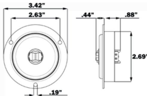
HOLE CUT-OUT: 2.75"
