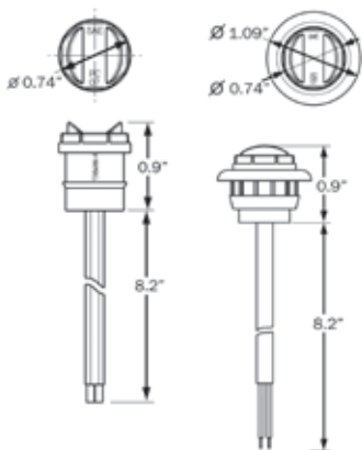
HOLE CUT-OUT: 0.75"
