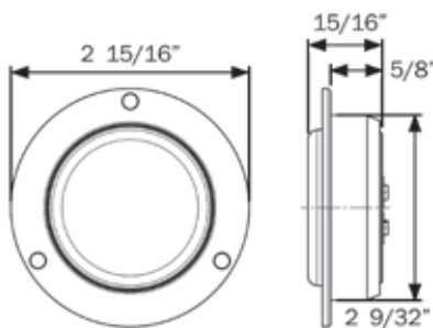
HOLE CUT-OUT: 2.313"
