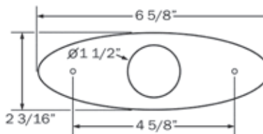
HOLE CUT-OUT: 1.5"
