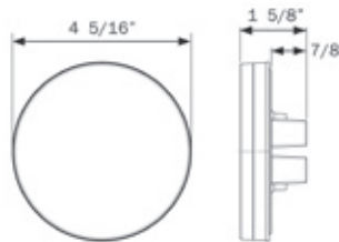
HOLE CUT-OUT: 4.5"
