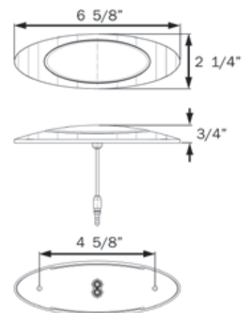
HOLE CUT-OUT: 1.5"
