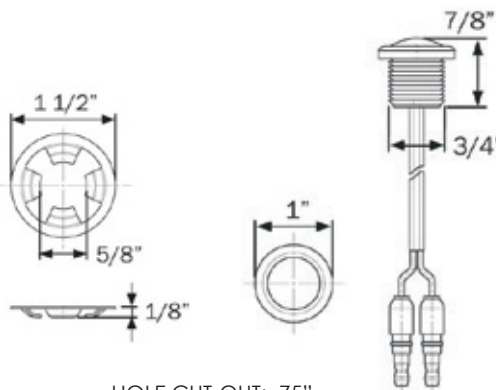
HOLE CUT-OUT: .75"
