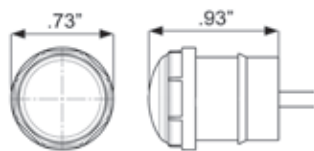
HOLE CUT-OUT: .75"
