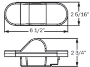
HOLE CUT-OUT: 6.85" X 2.5" (1.25" R)
